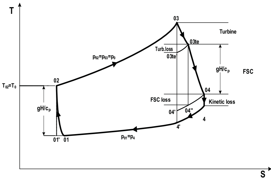
Fig. 7. The thermodynamic diagram of the SAEP
